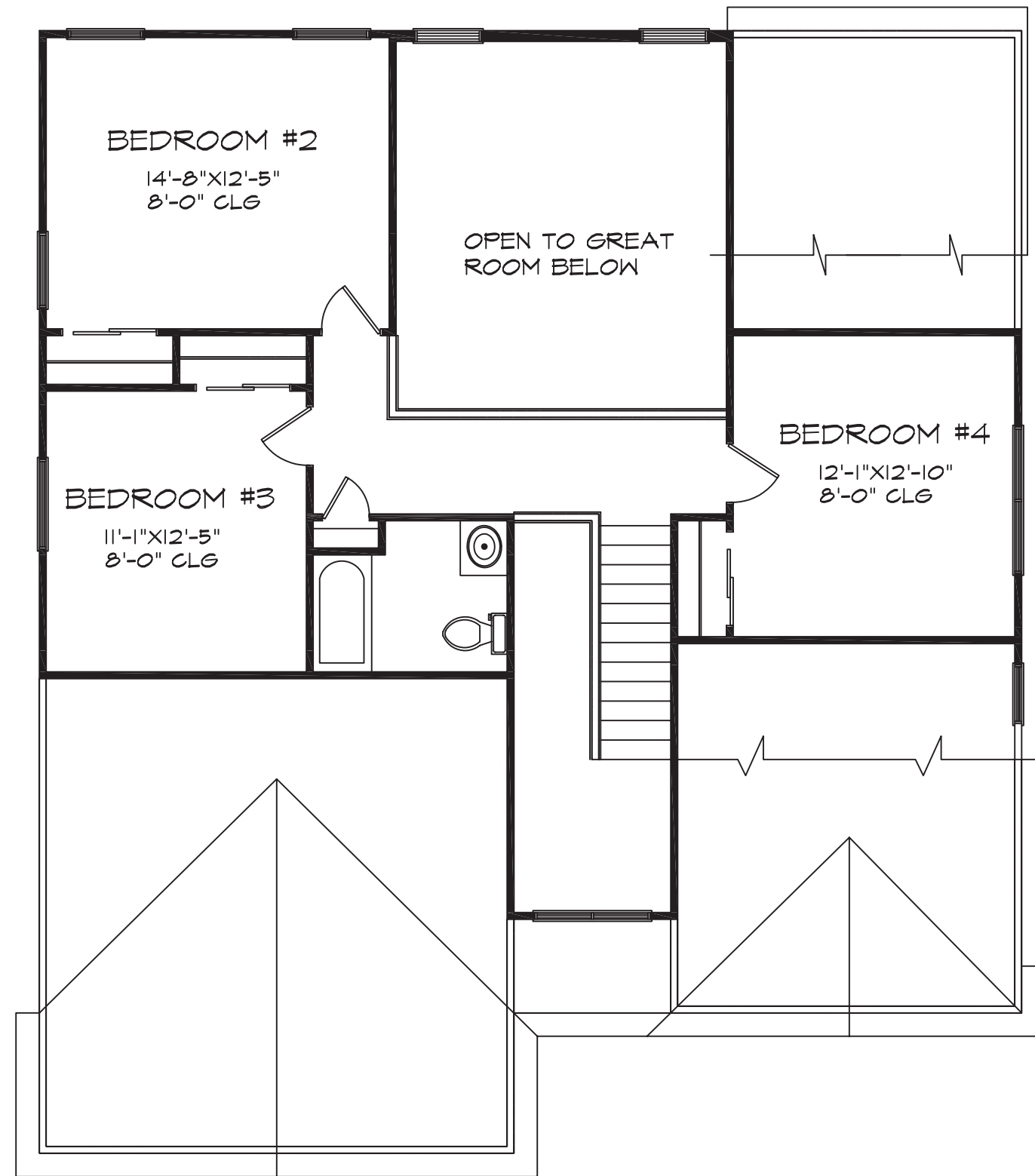
SECOND FLOOR
