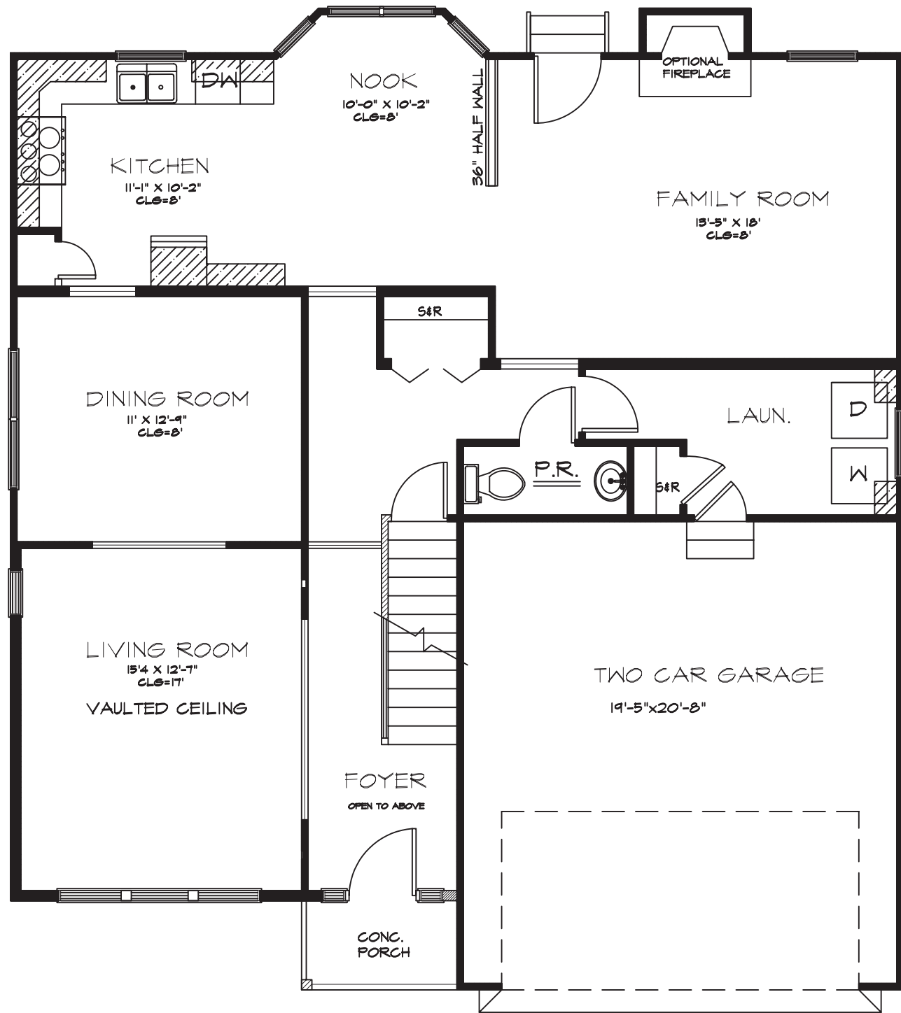
FIRST FLOOR
